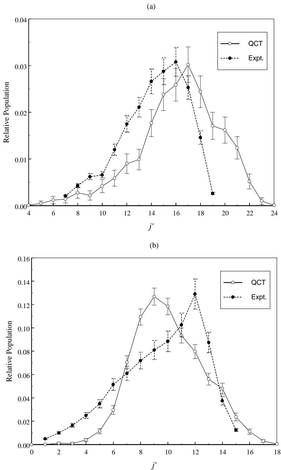
Figure 6. Same as Figs. 4 and 5, but for the HCl ( v = 2, j = 9 ) initial state. The QCT distributions are compiled from propagating a total of 280 000 trajectories, weighted by the collision energy distribution function of Fig. 3(a) and normalized as described in text.
