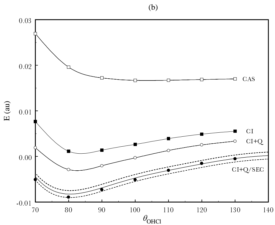
Figure 2. The angular dependence of the potential at (a) the saddle point values of (r_{\text{OH}}, r_{\text{HCl}}) and (b) at the values of (r_{\text{OH}}, r_{\text{HCl}}) corresponding to the minimum in Fig. 1(b). Smooth lines connect the ab initio data at the CAS, CI, and CI+Q levels of calculation. The CI+Q/SEC data are compared to the fitted surface itself, shown as the solid line, with the dashed lines above and below representing the limits V \pm \Delta V_{\text{rms}} .
